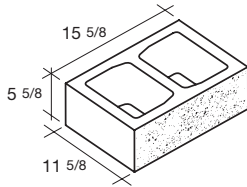
12x6x16 Standard
