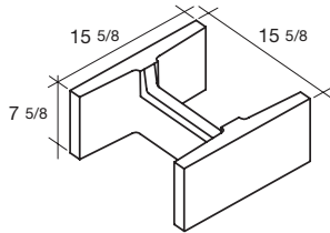
16x8x16 Double Open End Bond Beam
