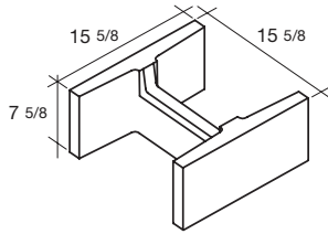
16x8x16 Double Open End Bond Beam
