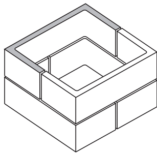
24x8x12 Alternate Coursing Running Bond
