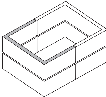
24x8x16 Coursing Stack Bond
