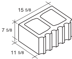
12x8x16 5-Flute 1-Side
