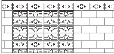
6x8x16 Grille-Lite 3
