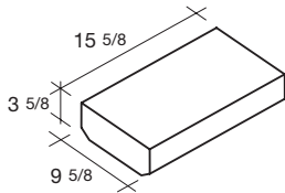
10x4x16 Beveled Cap
