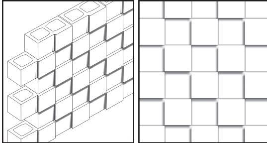
Projected Block Running Bond
