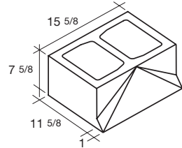
12x8x16 Shadow Block
