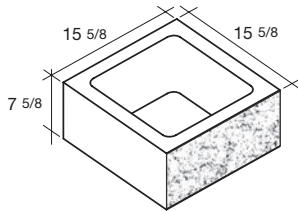
16x8x16 Ring Split 1-Side Special Order Only.
