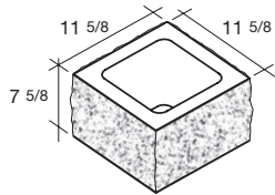
12x8x12 Ring Split 4-Sides Limited Inventory.
