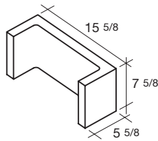
16x8x6 C-Alternate
