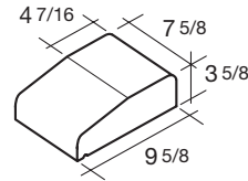
10x4x8 Flat Top Sill Block
