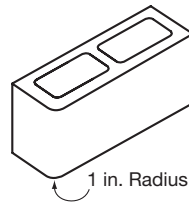
6x8x16 Standard Single Bullnose SPECIAL ORDER ONLY
