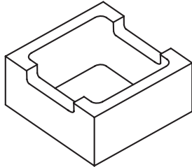
16x8x16 Ring Bond Beam SPECIAL ORDER ONLY
