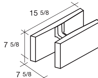
8x8x16 22.5-Degree Miter DOE BB Left and Right Also available in 6-inch wide. SPECIAL ORDER ONLY
