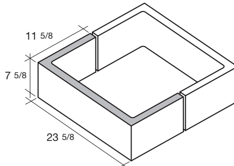
24x8x12 C-Alternate SPECIAL ORDER ONLY
