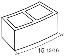
8x8x16 5-Foot 2-Inch Radius SPECIAL ORDER ONLY
