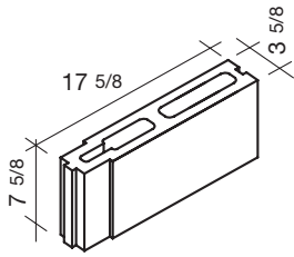
4x8x18 Catalina SPECIAL ORDER ONLY
