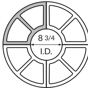
Ends of 1-Foot Radius are knock-out bond beams. I.D.
