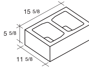
12x6x16 Standard SPECIAL ORDER ONLY
