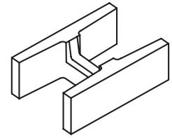
12x6x16 Double Open End Bond Beam SPECIAL ORDER ONLY
