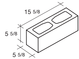
6x6x16 Standard SPECIAL ORDER ONLY
