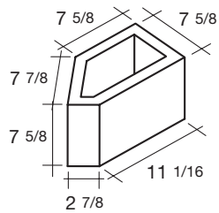
8x8x16 Corner 45-Degree SPECIAL ORDER ONLY
