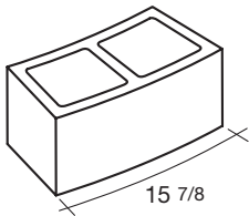
8x8x16 5-Foot 2-Inch Radius SPECIAL ORDER ONLY
