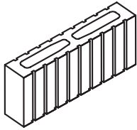
4x8x18 Open Top Balboa SPECIAL ORDER ONLY
