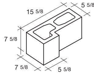
6x8x16 Corner 8-Inch Return SPECIAL ORDER ONLY
