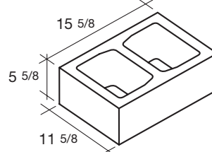
12x6x16 Standard SPECIAL ORDER ONLY
