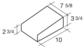
10x4x8 Sloped Sill Block
