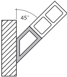
8x8x16 Standard 45-Degree SPECIAL ORDER ONLY
