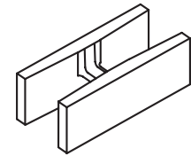
8x6x16 Double Open End Bond Beam SPECIAL ORDER ONLY
