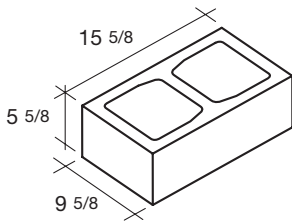
10x6x16 Standard SPECIAL ORDER ONLY
