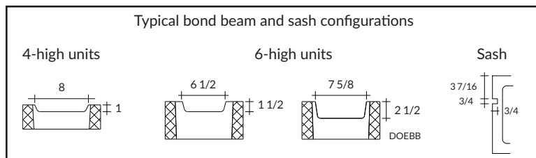
12x4x16 Open End Bond Beam
