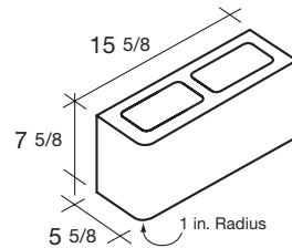
6x8x16 Standard Single Bullnose SPECIAL ORDER ONLY
