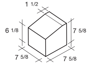
8x8x8 Sill Block
