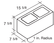
8x8x16 Standard Single Bullnose SPECIAL ORDER ONLY
