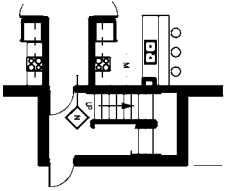
6 A10 ENLARGED MASONRY / PRECAST CONSTRUCTION PLAN SCALE: 1/8" = 1'-0"
