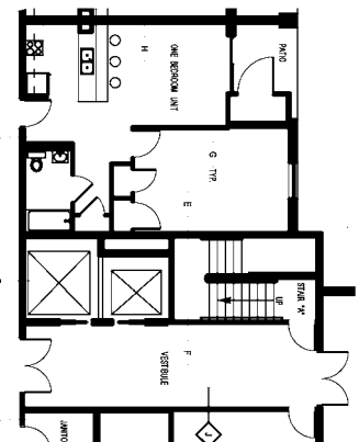
2 A10 ENLARGED METAL STUD CONSTRUCTION PLAN SCALE: 1/8" = 1'-0"
