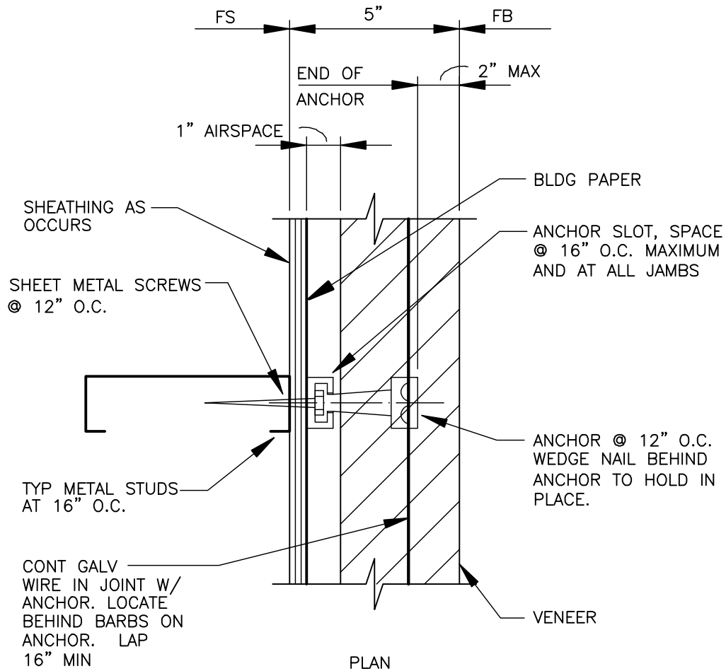
TYPICAL VENEER ANCHORAGE TO METAL STUDS
