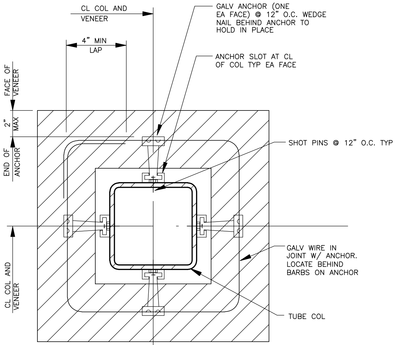
TYPICAL VENEER ANCHORAGE TO TS COLUMN
