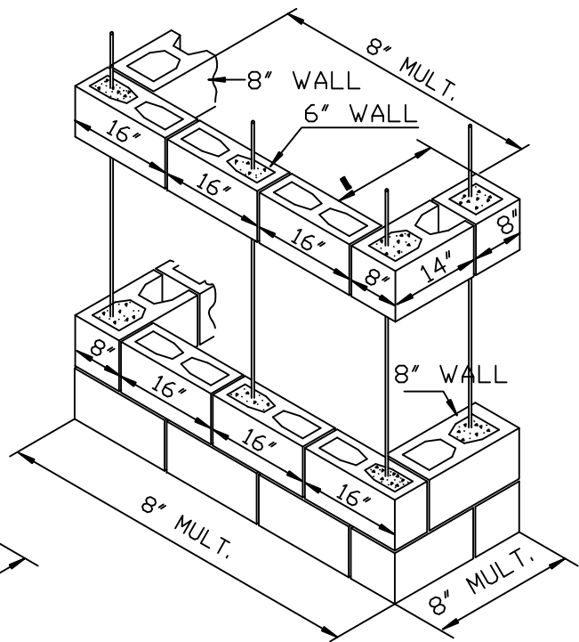
6" WALL TO 8" WALL
